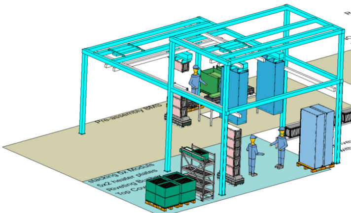
Abbildung 25 – BatteryPack-Montage
